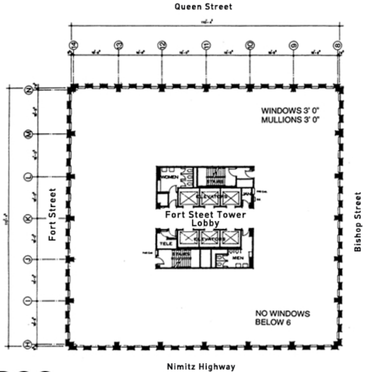
Fort Street Tower - Typical Floor Plan
